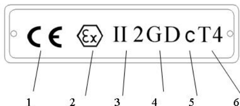
Fig. 7 Plaquette ATEX.
