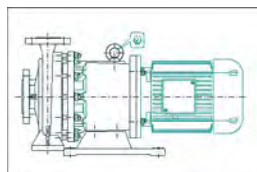
Fig. 10 Fabrication monobloc.
